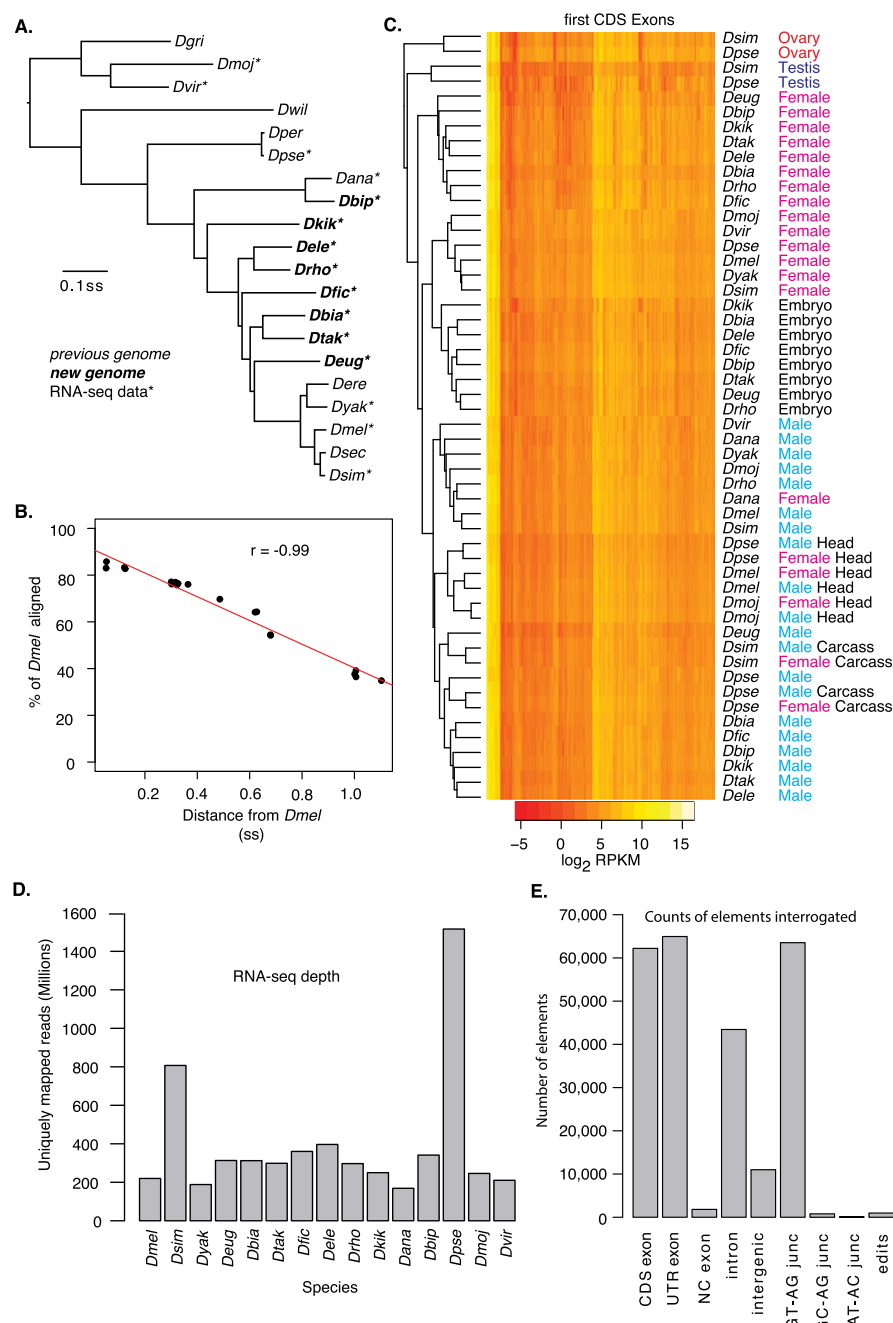
Figure 1. Genome assemblies and RNA-seq. (A) Bayesian phylogenetic tree of 20 sequenced Drosophila species (four letter abbreviations). All nodes are supported by 100% posterior probabilities. Scale bar indicates phylogenetic distance in substitutions per site (ss). Previously (italics) and newly assembled (bold italics) genomes, and those with supporting RNA-seq data (asterisk) are indicated. (B) Scatterplot showing alignment versus phylogenetic distance from D. melanogaster (linear trendline in red). (C) Heatmap and hierarchical clustering of expression values for 3223 first coding exons from the indicated samples. Adult ovary (dark red) and testis (dark blue) included developing germ cells and somatic gonadal cells and internal reproductive tracts derived from the genital disc. Females (pink) and males (light blue) were whole adults, embryos were unsexed, heads were from adults, and carcasses were all adult tissues remaining after removal of the gonads and internal reproductive tract. RPKM scale is shown for 15 species. The distance scale for hierarchical leaves was arbitrary. (D) Sequencing depth by species. A limited number of RNA-seq reads from heads (20.5 million reads for D. melanogaster , 28.4 million reads for D. pseudoobscura , and 51.6 million reads for D. mojavensis ) were previously published (Graveley et al. 2011). The remaining reads are reported here for the first time. (E) The number of each element type from the modENCODE version 2 (MDv2) annotation. We examined the conserved sequence and expression characteristics of all such elements. For purposes of analysis, exons with both UTR and CDS sequences were split.
