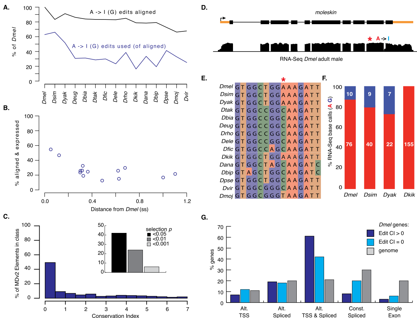
Figure 8. RNA editing. (A) D. melanogaster editing events that align to the indicated genomes (black) and are used if aligned (blue). (B) Combined sequence and expression conservation for editing events. (C) Frequency of conservation index scores for MDv2-annotated edits. (Inset) Probability that CI is random (shades of black). (D) An example of a validated editing site in moleskin with a low CI. Gene model and log 2 scale RNA-seq coverage in adult males with editing site are indicated (red asterisk). (E) Genome alignment of moleskin editing site (red asterisk) and flanking region. (D,E) Nucleotides are color coded (I, light blue; A, red; G, green; C, blue; T, orange). (F) Stacked bar plot of editing site base calling in D. melanogaster , D. simulans , D. yakuba , and D. kikkawai . (G) Frequencies of editing occurrence among transcripts from genes with annotated alternative transcription start sites (Alt. TSS), alternative splicing (Alt. Spliced), both alternative transcription start sites and splicing (Alt. TSS & Alt. Spliced), multiexon genes with a single annotated isoform, and single exon genes. All D. melanogaster genes (gray), those with edits in at least one other species (dark blue), and those with edits only in D. melanogaster (light blue) are shown.
