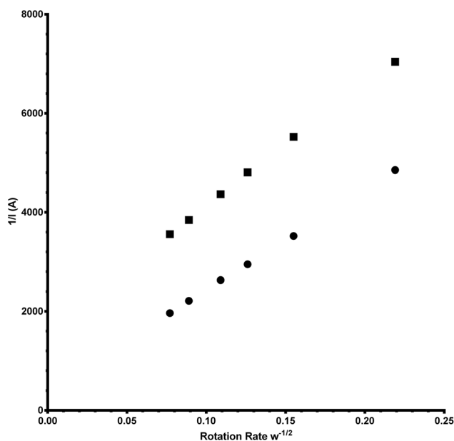
Fig. 15 Koutecký–Levich (K–L) plots for the Pt-ring Pt-disk (circles) and the Pt-ring GC-disk (squares) control RRDEs.
