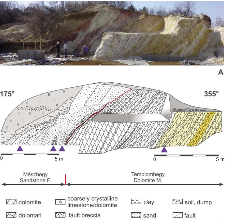
Fig. 5 Stratigraphic section of the southern part of the construction site in Villány. Light yellow color indicates fossiliferous beds and blue triangles refer to the screen-washed horizons. Among these, the dolomarl bed indicated with dark yellow color was the most productive one. This bed continues in the northern section (see Fig. 3)
