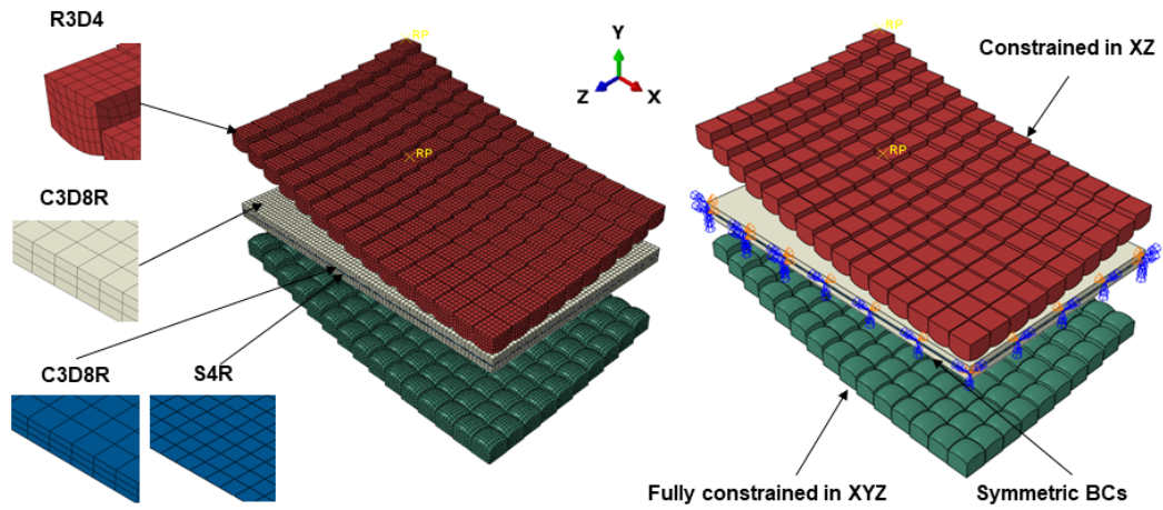
Figure 4: Schematic of the initial FE model, including element type and boundary conditions (BCs).
