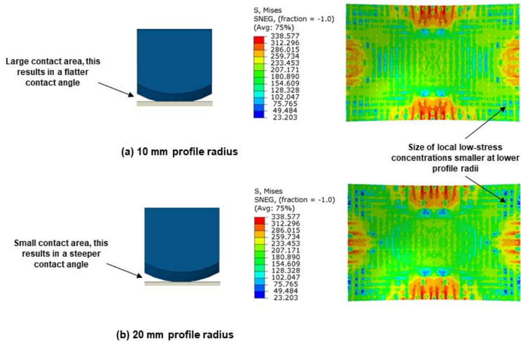
Figure 8: Comparison of the pin-to-cushion contact points and equivalent stress contours (S4R) on the upper workpiece surface when using 10 mm profile radius and 20 mm profile radius.
