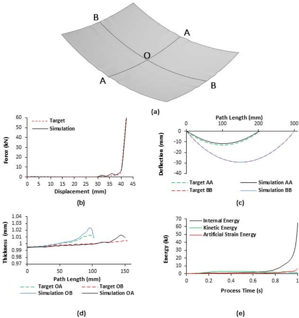
Figure 6: (a) Schematic overviewing principal axes of the deformed workpiece. (b) The force-displacement output of the C3D8R FE model compared to the target profile. (c) Deformed profile output of C3D8R FE model across principal axes compared to the target profile. (d) Thickness distribution output of S4R FE model across principal axes to centroid compared to the target distribution. (e) Energy history output of the C3D8R FE model.
