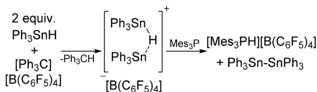
Scheme 4. Hydride abstraction from Ph_3SnH using [Ph_3C][B(C_6F_5)_4] and subsequent reaction with PMes_3 .
