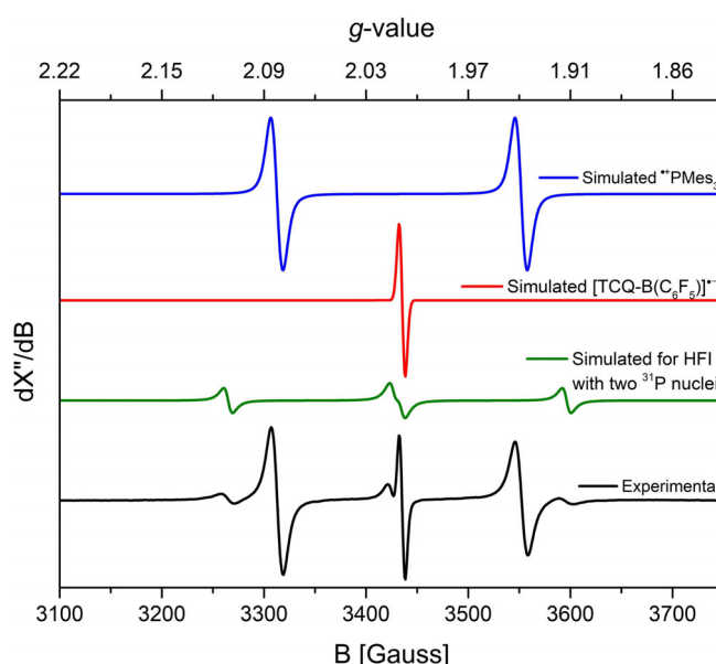
Figure 3. Experimental EPR spectrum (bottom) for reaction of \text{PMes}_3 , \text{B}(\text{C}_6\text{F}_5)_3 and TCQ (2:2:1) and simulated spectra for \text{PMes}_3^+ , \text{TCQ-B}(\text{C}_6\text{F}_5)_3^- and the third smaller signal. See the Supporting Information for experimental and simulation parameters. HFI = hyperfine interaction.
