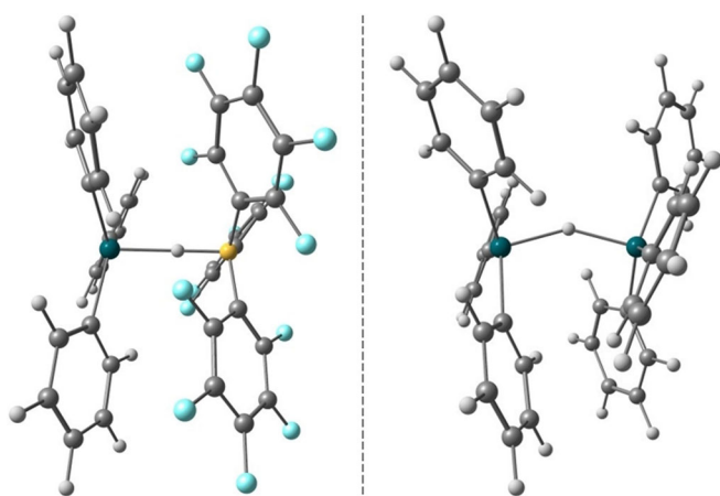
Figure 1. Computed structure for the adducts of Ph_3SnH with B(C_6F_5)_3 (left) and Ph_3Sn^+ (right) featuring a bridging hydride (DFT: \omega B97X-D/def2-TZVP ). Selected bond lengths and angles: Ph_3Sn-H-B(C_6F_5)_3 : Sn-H 1.83 Å, B-H 1.37 Å, Sn-H-B 180°. [Ph_3Sn-H-SnPh_3]^+ : Both Sn-H 1.87 Å; Sn-H-B 147°.
