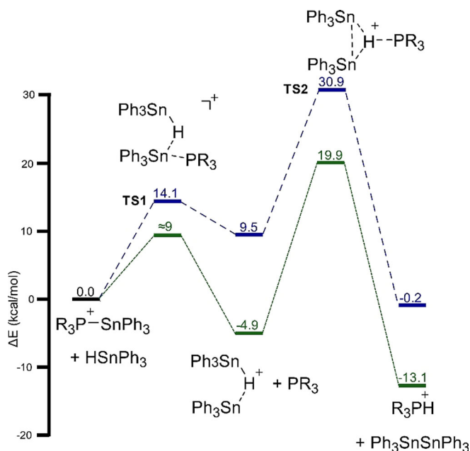
Figure 2. Proposed reaction mechanism based on DFT calculations at the \omega B97X-D/def2-TZVP level of theory. R = tBu (blue, dashed) or Mes (green, dotted). [HB(C_6F_5)_3]^- anion has been omitted for clarity. Energies in kcal mol ^{-1} .
