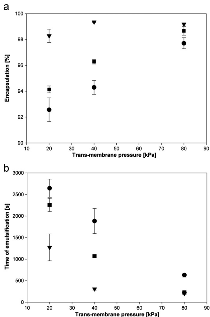
Fig. 6. Cross-flow membrane; (a) salt encapsulation in duplex emulsions measured just after emulsification and (b) time of batch emulsification. Effect of TMP and CFV: ( \nabla ) 0.11 \text{ m s}^{-1} , ( \blacksquare ) 0.17 \text{ m s}^{-1} and ( \bullet ) 0.22 \text{ m s}^{-1} .
