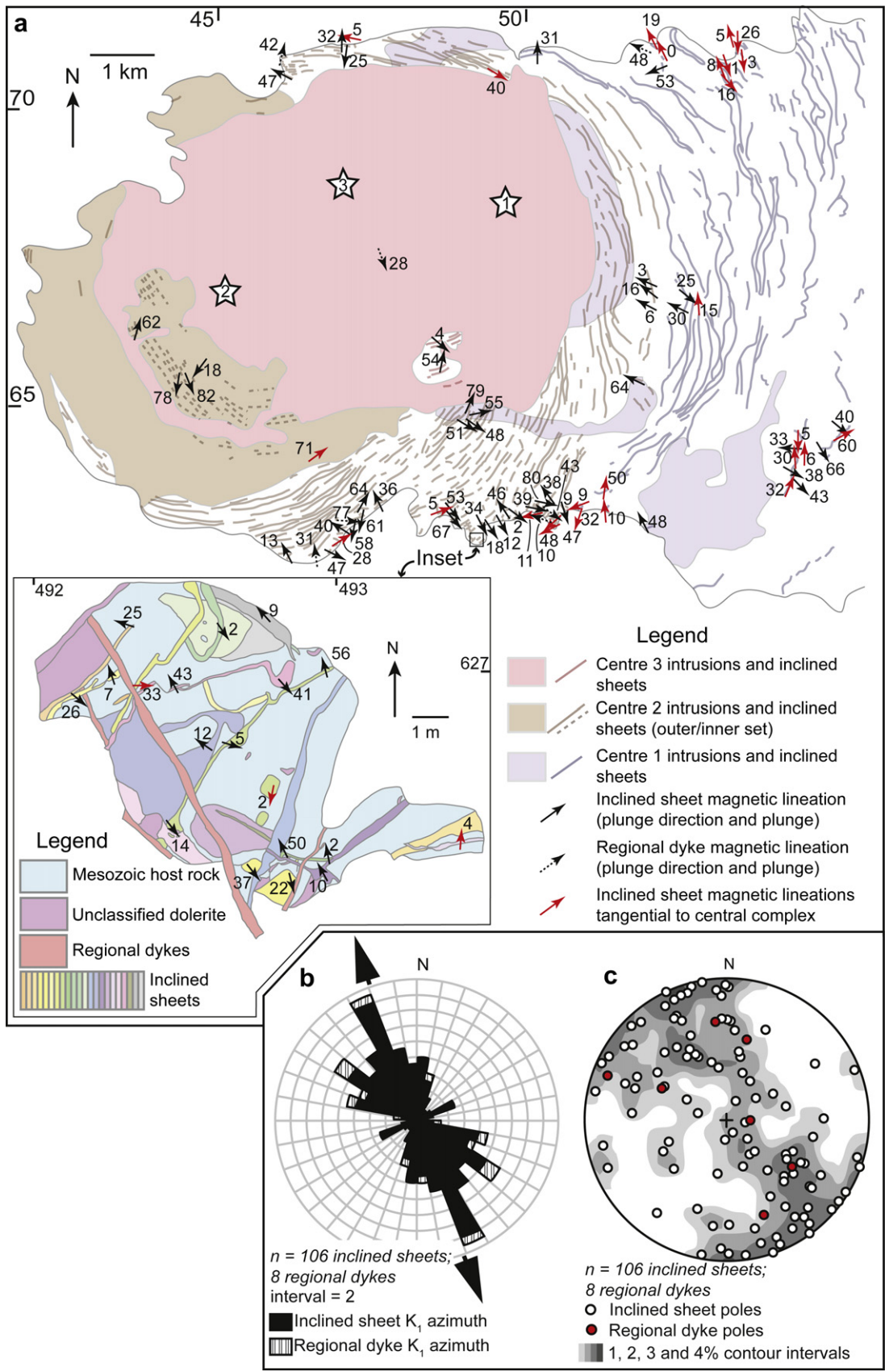
Fig. 8. (a) Map of the Ardnamurchan inclined sheets and the magnetic lineations (b) Rose diagram of all K_1 axes, with a strong NW–SE trend. (c) Equal-area stereographic projection of K_1 lineations showing a NW–SE trend and preponderance of sub-horizontal to moderately inclined plunges.
