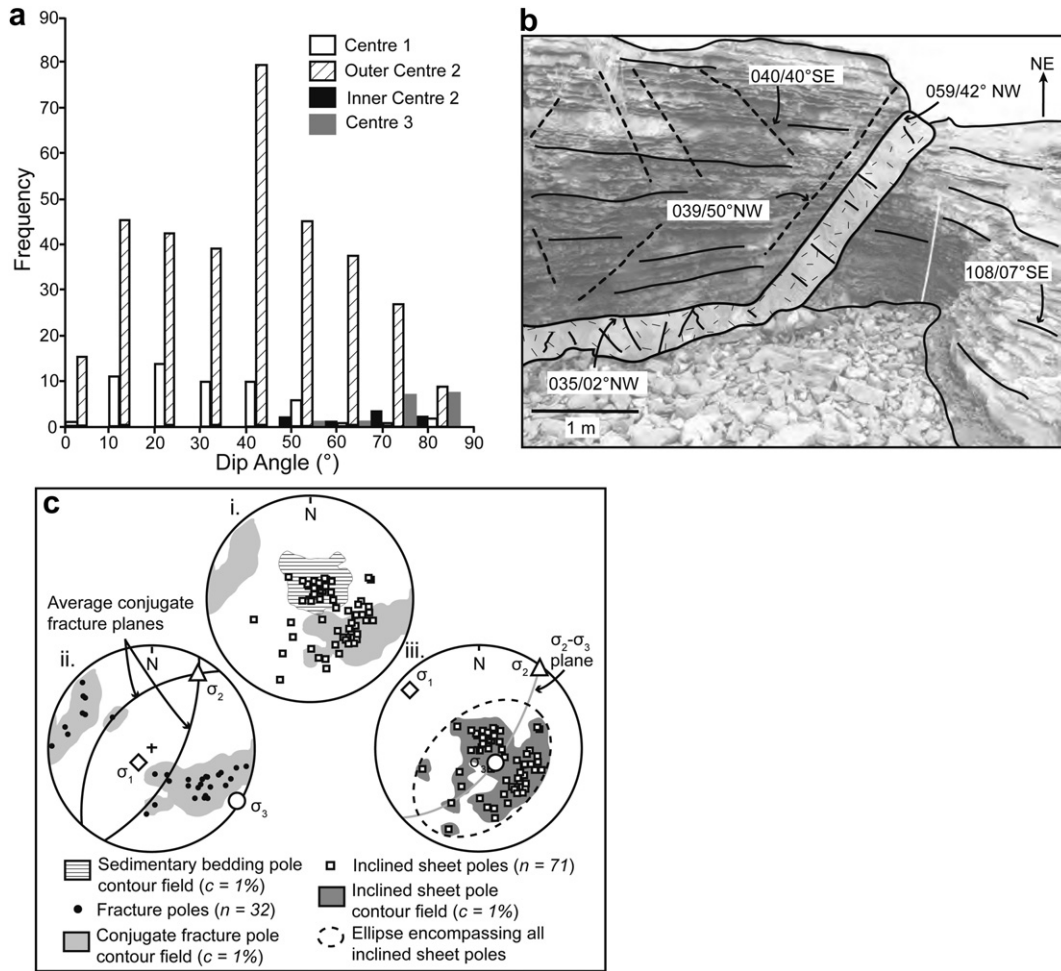
Fig. 4. (a) Dip versus frequency plot for the Ardnamurchan inclined sheets. (b) Transgressive sheet intruding bedding and also ramping up stratigraphy parallel to a series of inward-dipping fractures, one half of a conjugate fracture set (dashed lines) [NM 49240 62694]. (c) i) Equal-area stereographic projection of inclined sheet poles, conjugate fracture pole contours and bedding pole contours from Area 1 (Fig. 2). ii) Resolved formational principal stress axes orientations for conjugate fractures and iii) inclined sheet intrusion.
