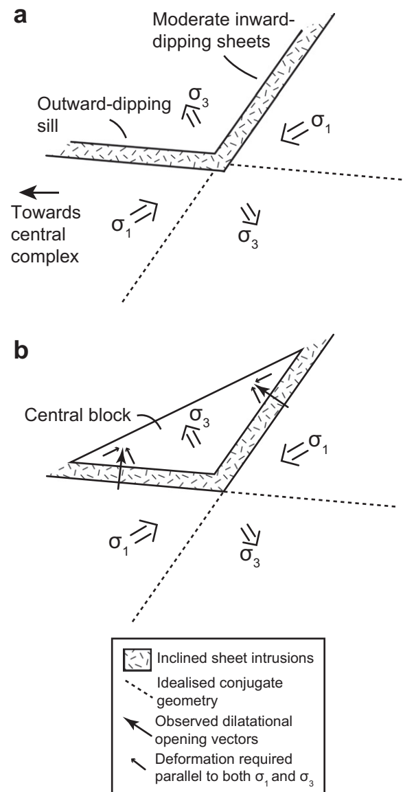
Fig. 10. Schematic cross-sections of the (a) conjugate nature of the outward- and inward-dipping inclined sheet segments defining an inwardly inclined \sigma_1 principal stress axis. (b) Highlights the required deformation of an uplifted central block given the dilatational opening vectors of the inclined sheets.
