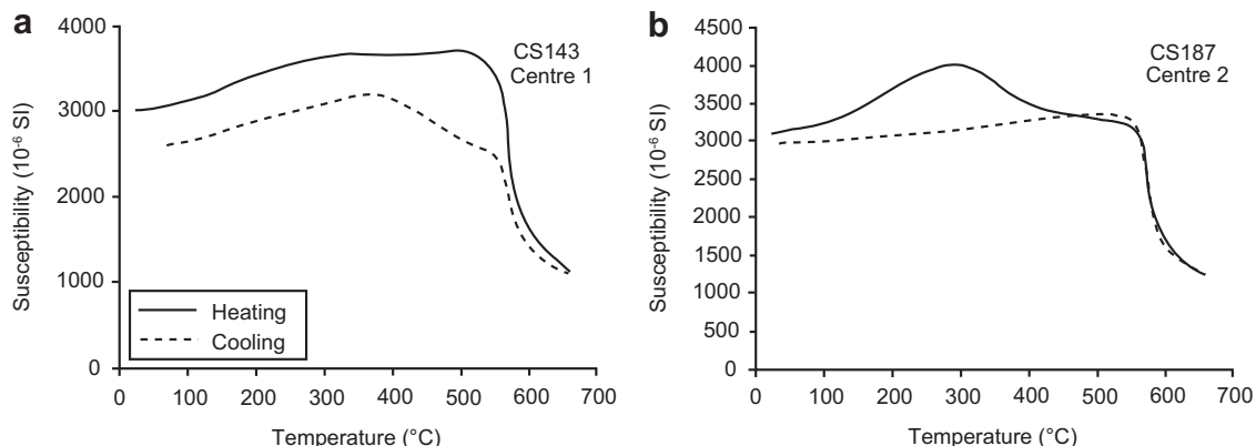
Fig. 6. High-temperature, low-field magnetic susceptibility experiment results. See text for details.
