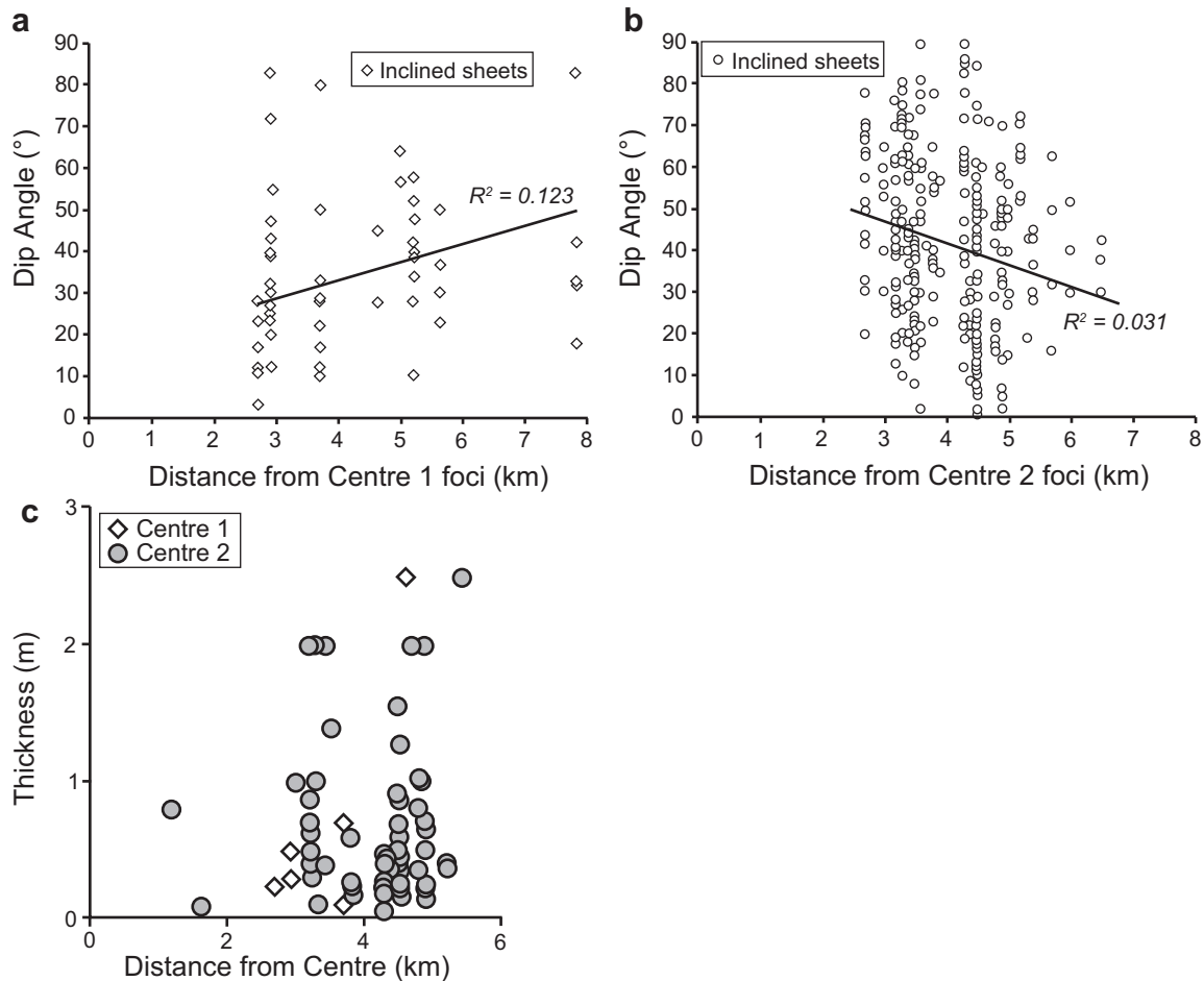
Fig. 5. (a) and (b) Plots of inclined sheet dip against distance from Centre 1 and 2 respectively. (c) A weak positive correlation between inclined sheet thickness and distance from the central complex.
