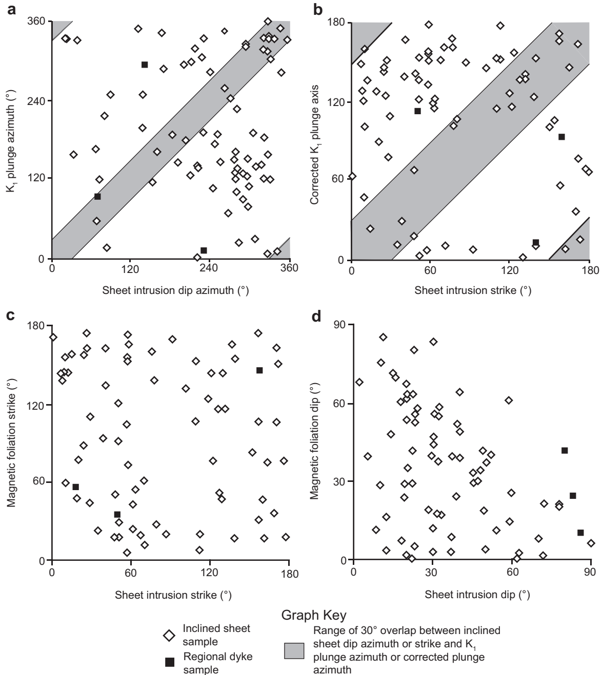
Fig. 9. (a) and (b) Graphs highlighting the weak correlation between K_1 azimuth and inclined sheet dip azimuth and strike. The corrected K_1 azimuths, for correlation with inclined sheet strike, ignore plunge direction and were converted to <180^\circ if required. (c) and (d) Plots showing the lack of relationship between the magnetic foliation and the orientation of the inclined sheets.
