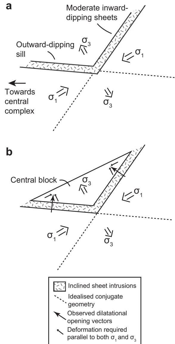
Fig. 10. Schematic cross-sections of the (a) conjugate nature of the outward- and inward-dipping inclined sheet segments defining an inwardly inclined \sigma_1 principal stress axis. (b) Highlights the required deformation of an uplifted central block given the dilatational opening vectors of the inclined sheets.
