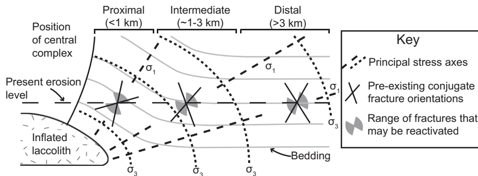
Fig. 11. Sketch of local principal axes orientations formed in response to an inflating laccolith and the resultant fracture/bedding planes that are reactivated. Proximal to the laccolith only steep fractures are reactivated and at an intermediate distance, where most of the Ardnamurchan inclined sheets are situated, intrusion exploits both moderate inward-dipping fractures and bedding planes. Distally, bedding planes are predominantly intruded.
