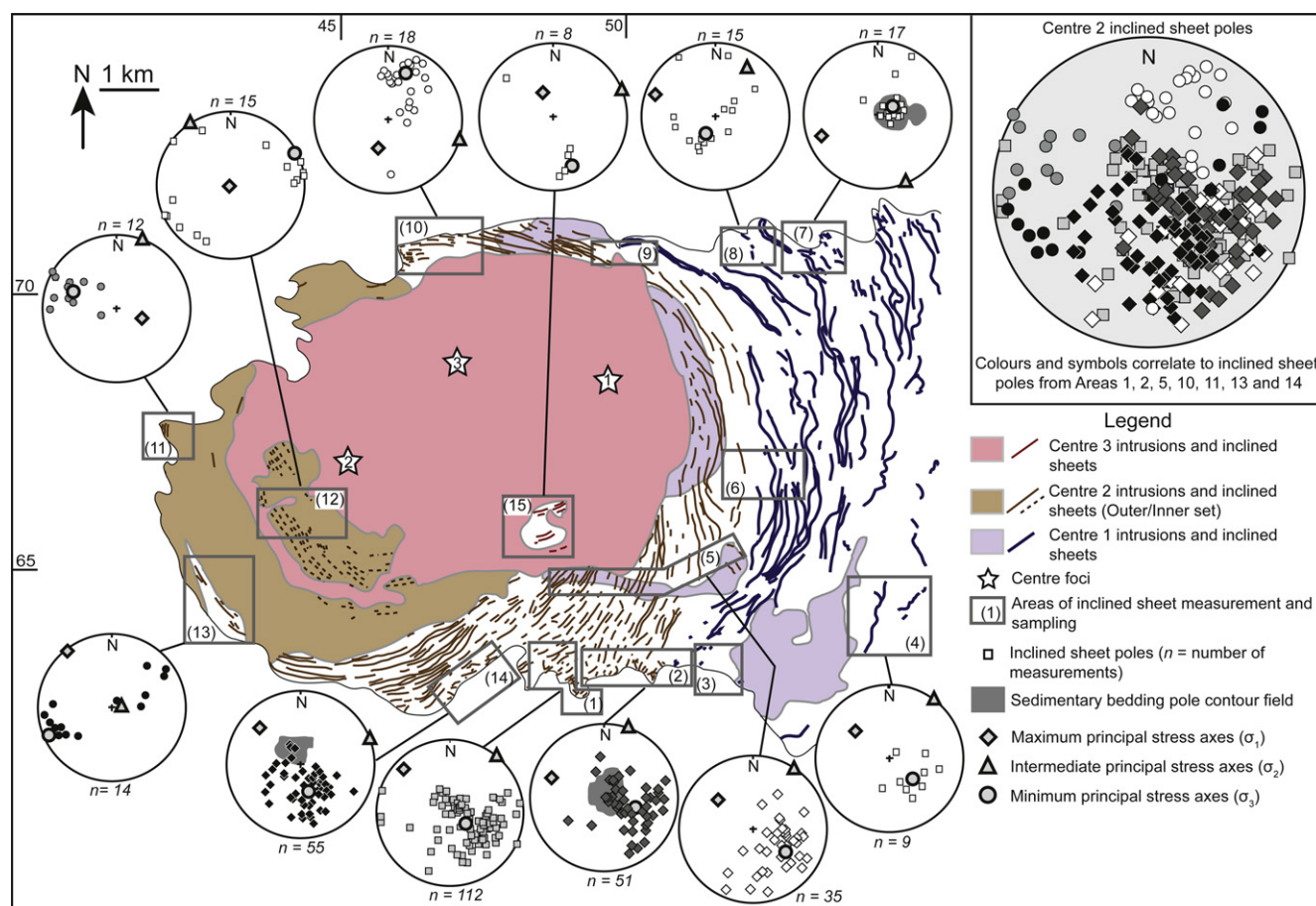
Fig. 2. Detailed map of Ardnamurchan depicting accentuated inclined sheet strikes. Areas of main data collection are shown (adapted from Richey and Thomas, 1930; Emeleus, 2009). Equal-area lower-hemisphere stereoplots of inclined sheet poles are presented highlighting their variability in dip value and dip azimuth, although on average their dip disposition is towards the central complex. A combined plot of all Outer Centre 2 inclined sheet poles is inset. Bedding pole contour fields and principal stress axes, resolved from the inclined sheet poles, are also displayed. The \sigma_1 stress axes are often oriented towards the central complex and become steeper as proximity to the centre increases, indicating a radially inwardly inclined orientation. Conversely, \sigma_3 becomes shallower with distance from the central complex. Grid references refer to the UK National Grid co-ordinate system.
