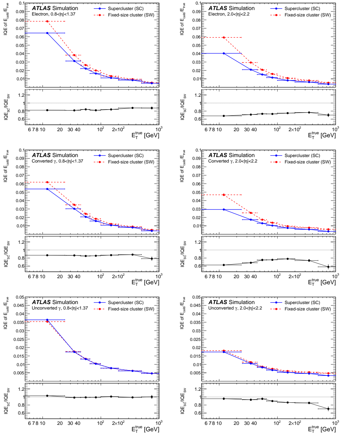
Figure 7. Calibrated energy response resolution, expressed in terms of IQE, for electrons (top), converted photons (middle), and unconverted photons (bottom) simulated with \langle \mu \rangle = 0 . Two representative pseudorapidity ranges are shown. The response resolution for fixed-size clusters based on the sliding window method is shown in dashed red, while the supercluster-based response resolution is shown in full blue. For all plots, the bottom panel shows the ratios between the IQE obtained using the supercluster reconstruction and using the sliding window method.
